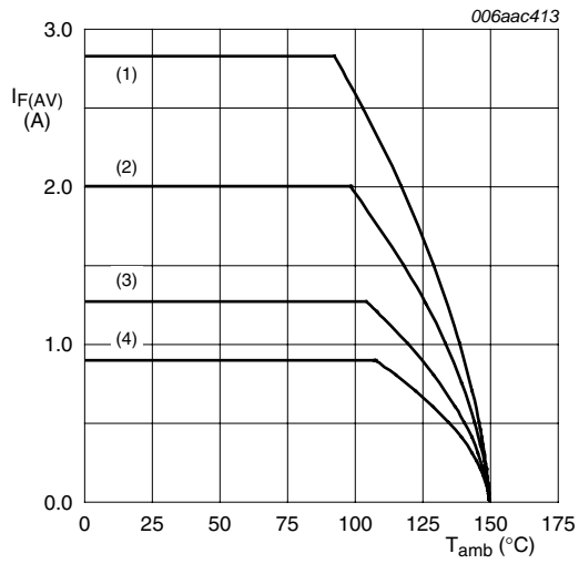
Ceramic PCB, Al_2O_3 , standard footprint T_j = 150^{\circ}C (1) \delta = 1 ; DC (2) \delta = 0.5 ; f = 20 kHz (3) \delta = 0.2 ; f = 20 kHz (4) \delta = 0.1 ; f = 20 kHz
